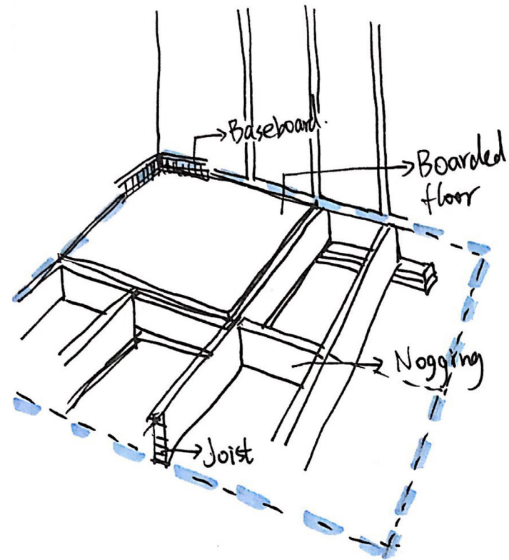
Floor Construction.
