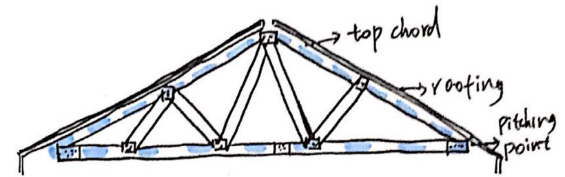
Roof truss
