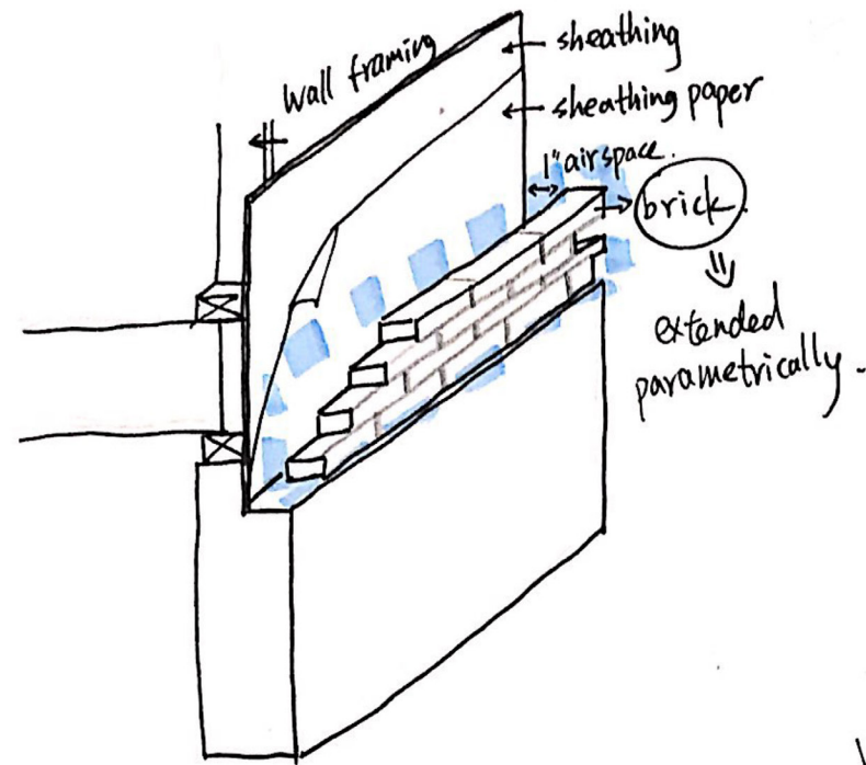
Brick Veneer Wall.
